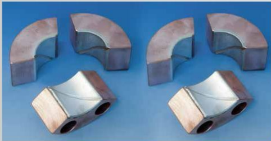
高純度導電體銀瓦片 High purity conductivity of silver brush
